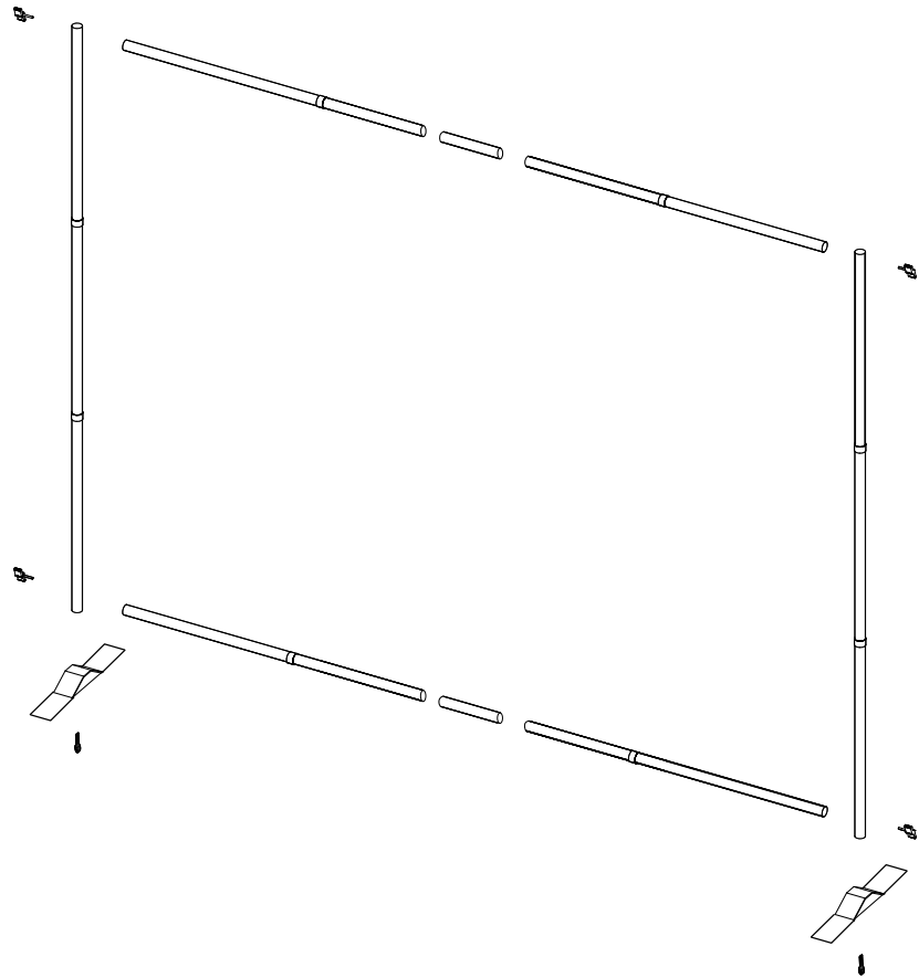
Exploded View
